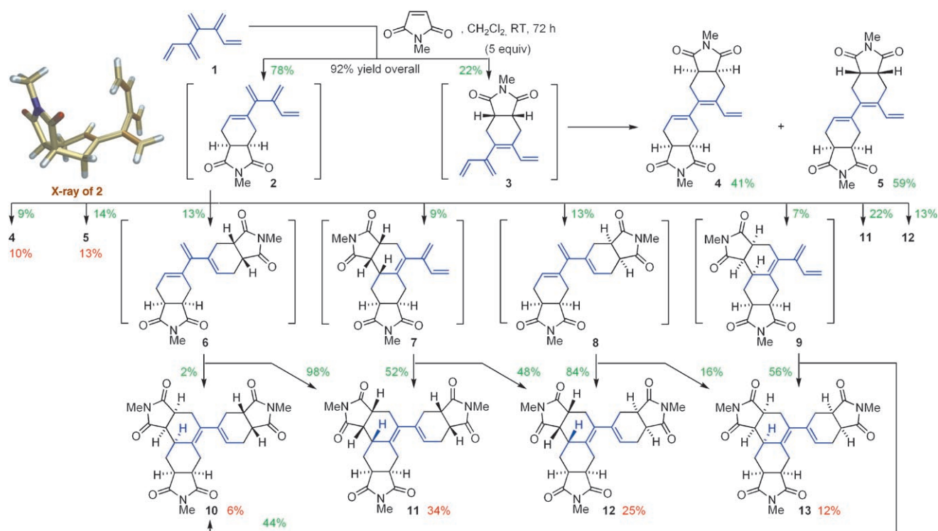
Scheme 3. Reaction of [5]dendralene with NMM. (Red = product breakdown (%) for reaction of 1 with excess NMM. Green = product breakdown (%) for reactions with 1:1 precursor/NMM stoichiometry.) X-ray structure of 2 : red O, blue N, yellow C, white H. X-ray crystal structures of 4 , 7 , and 10–13 can be found in the Supporting Information.
